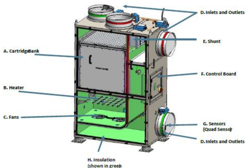
Figure 13: Cutaway view of York EcoAdvance 100E
