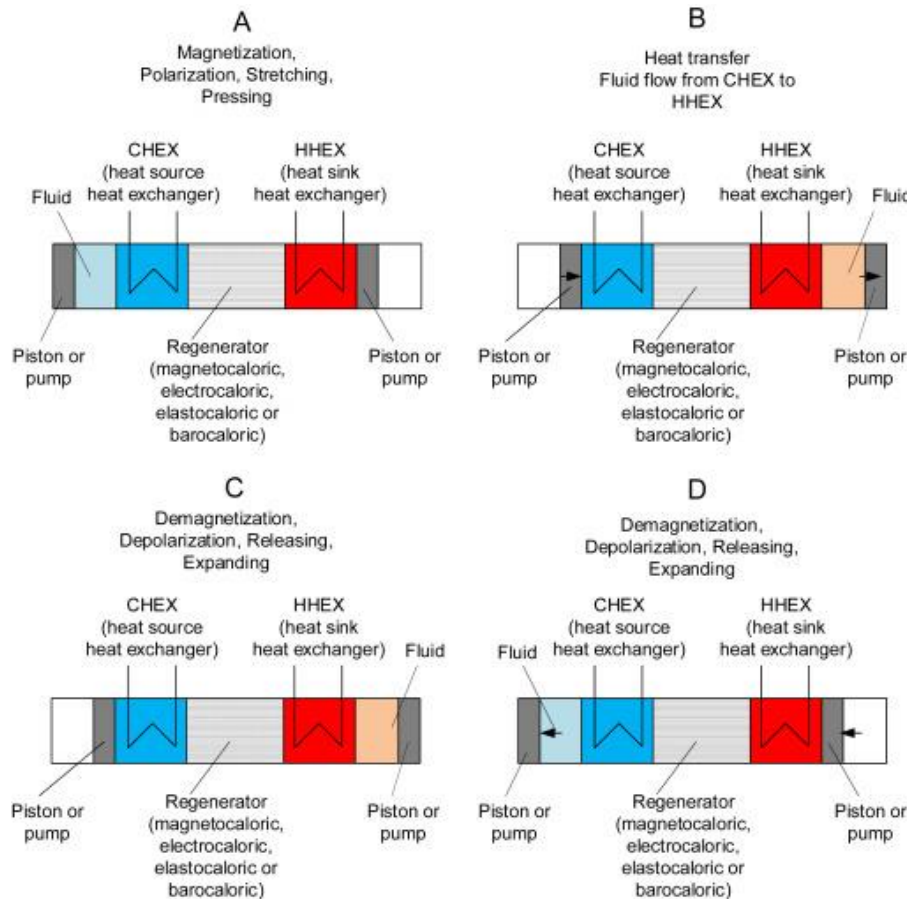
Figure 21: Schematic of active electrocaloric regeneration heat pump process
