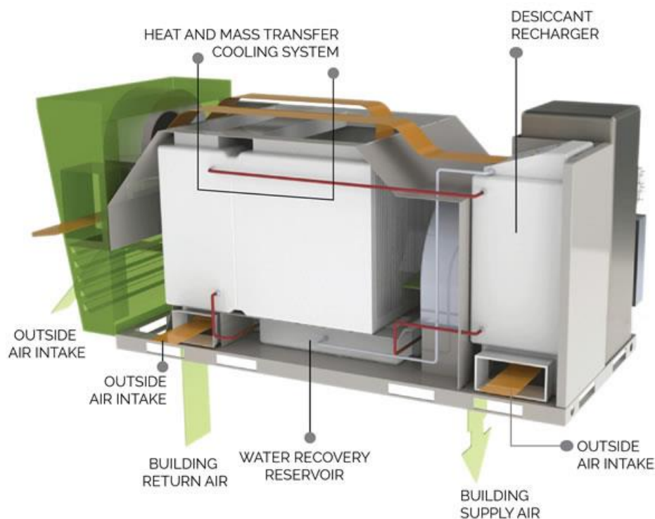
Figure 31: Illustration of BePowerTech RTU product
