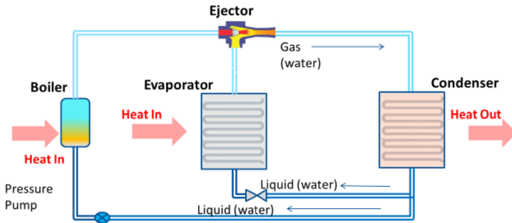
Figure 28: Steam ejector heat pump system
