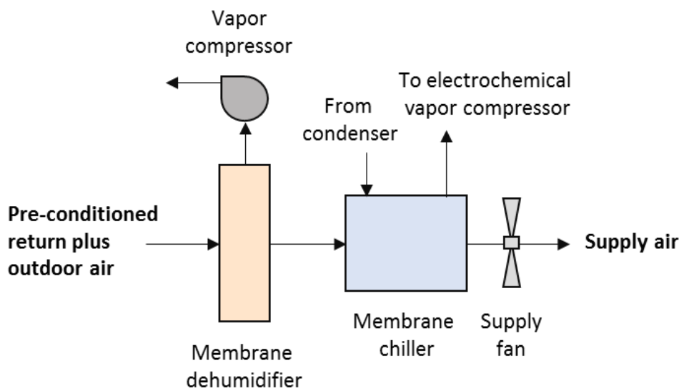
Figure 15: Schematic of membrane cooling system
