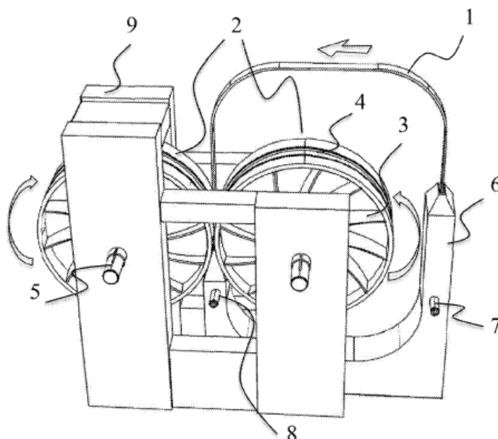
Figure 19: Illustration of prototype thermoelastic cooling system
