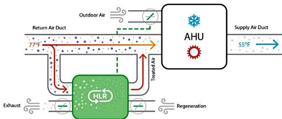
Figure 12: Schematic of ventilation reduction through advanced filtration
