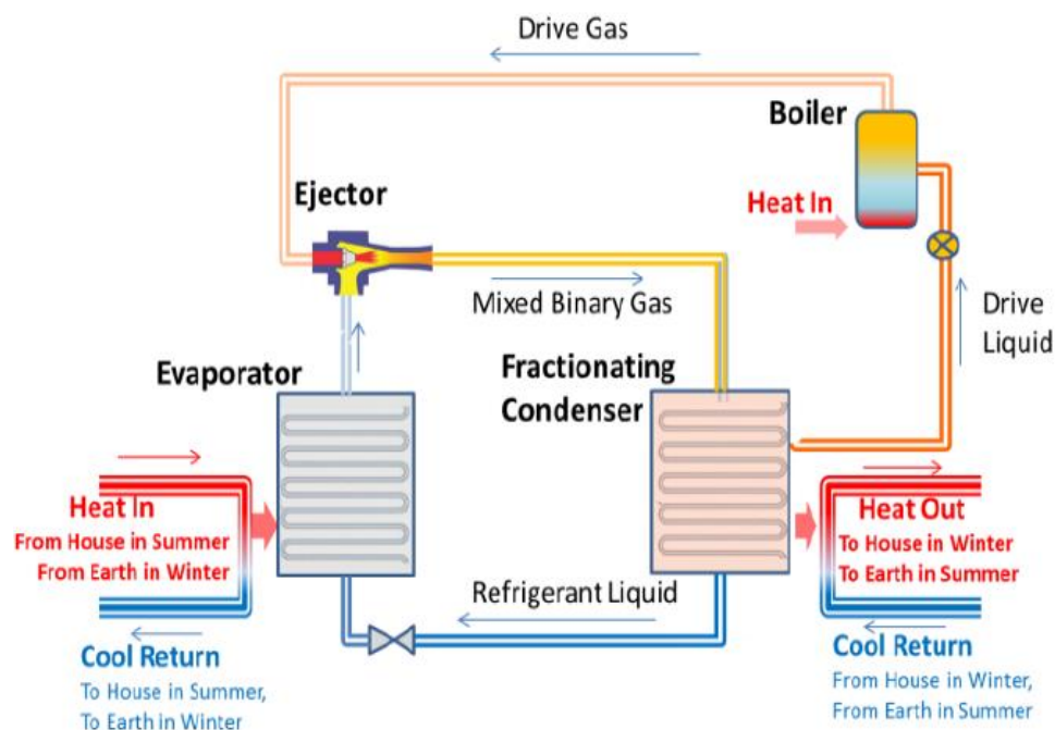
Figure 29: Binary fluid ejector heat pump system
