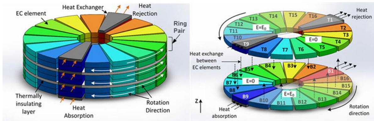
Figure 22: Schematic of rotary electrocaloric cooling system
