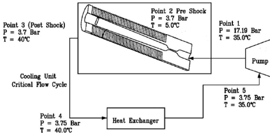
Figure 17: Schematic of an MCFC system
