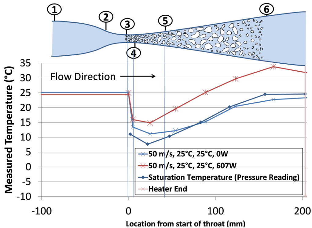
Figure 16: Measured temperatures in an experimental MCFC nozzle
