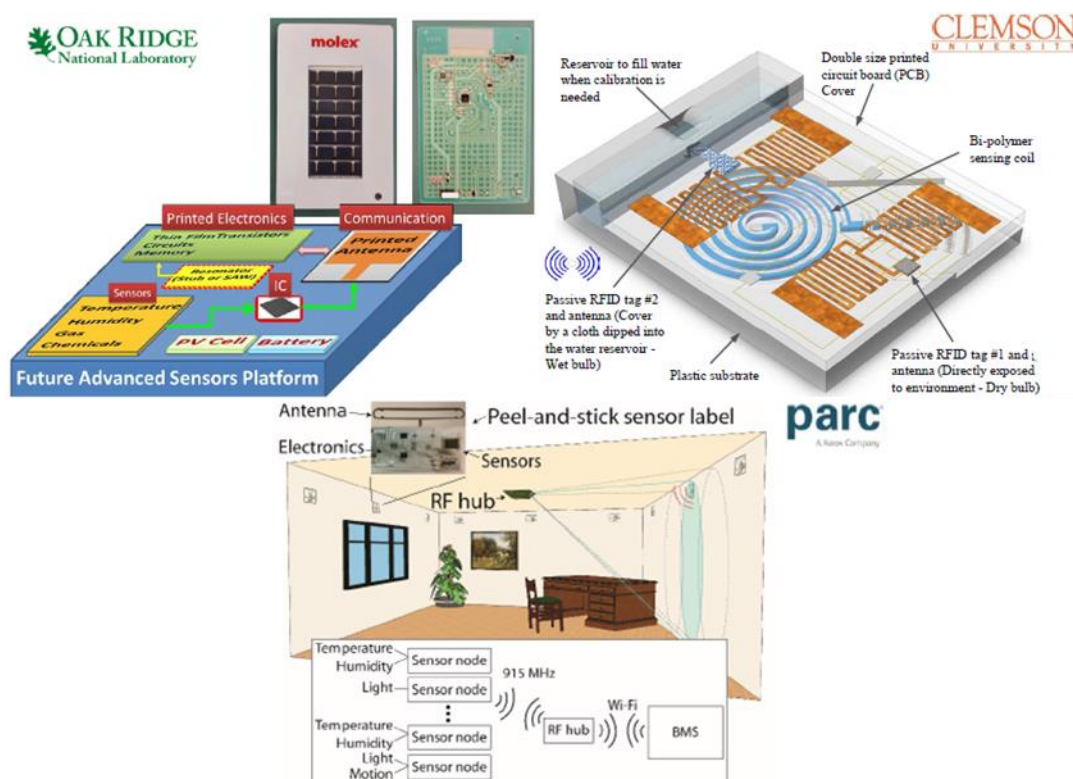
Figure 10: Examples of multifunction plug-and-play wireless sensors
