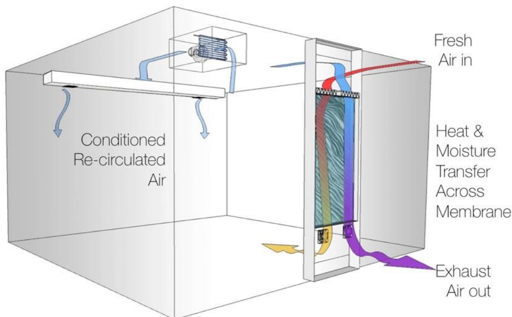
Figure 11: Building-integrated heat and moisture exchange panels
