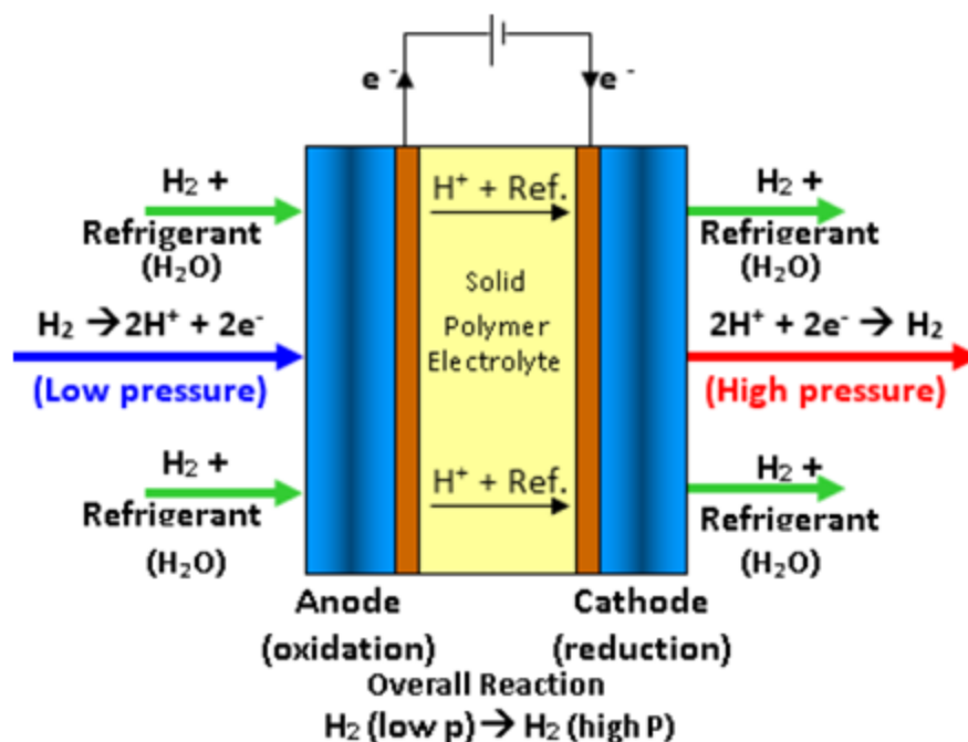
Figure 23: Electrochemical compressor diagram
