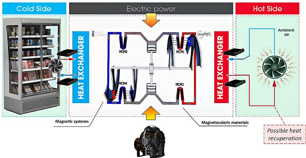
Figure 24: Schematic of fluid-based magnetic cooling concept
