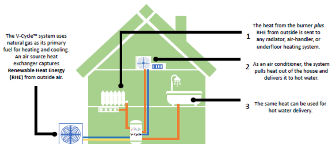
Figure 27: Schematic of ThermoLift VHP in residential application
