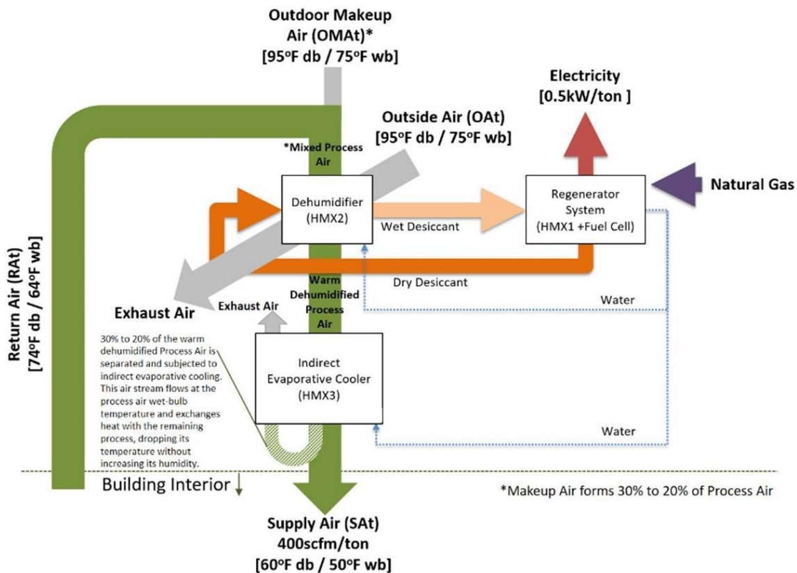
Figure 30: Process diagram of fuel cell combined cooling, heating, and power system
