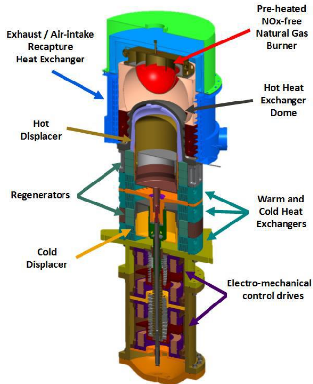
Figure 26: Cutaway view of ThermoLift VHP
