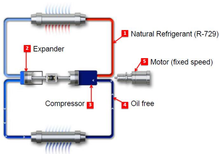
Figure 20: Schematic of S-RAM heat pump concept
