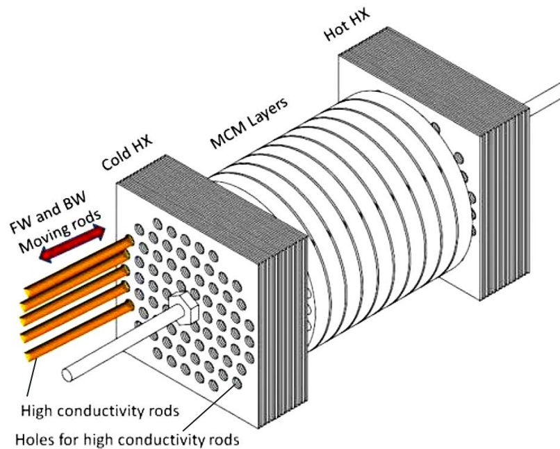
Figure 25: Schematic of solid-state magnetic cooling concept
