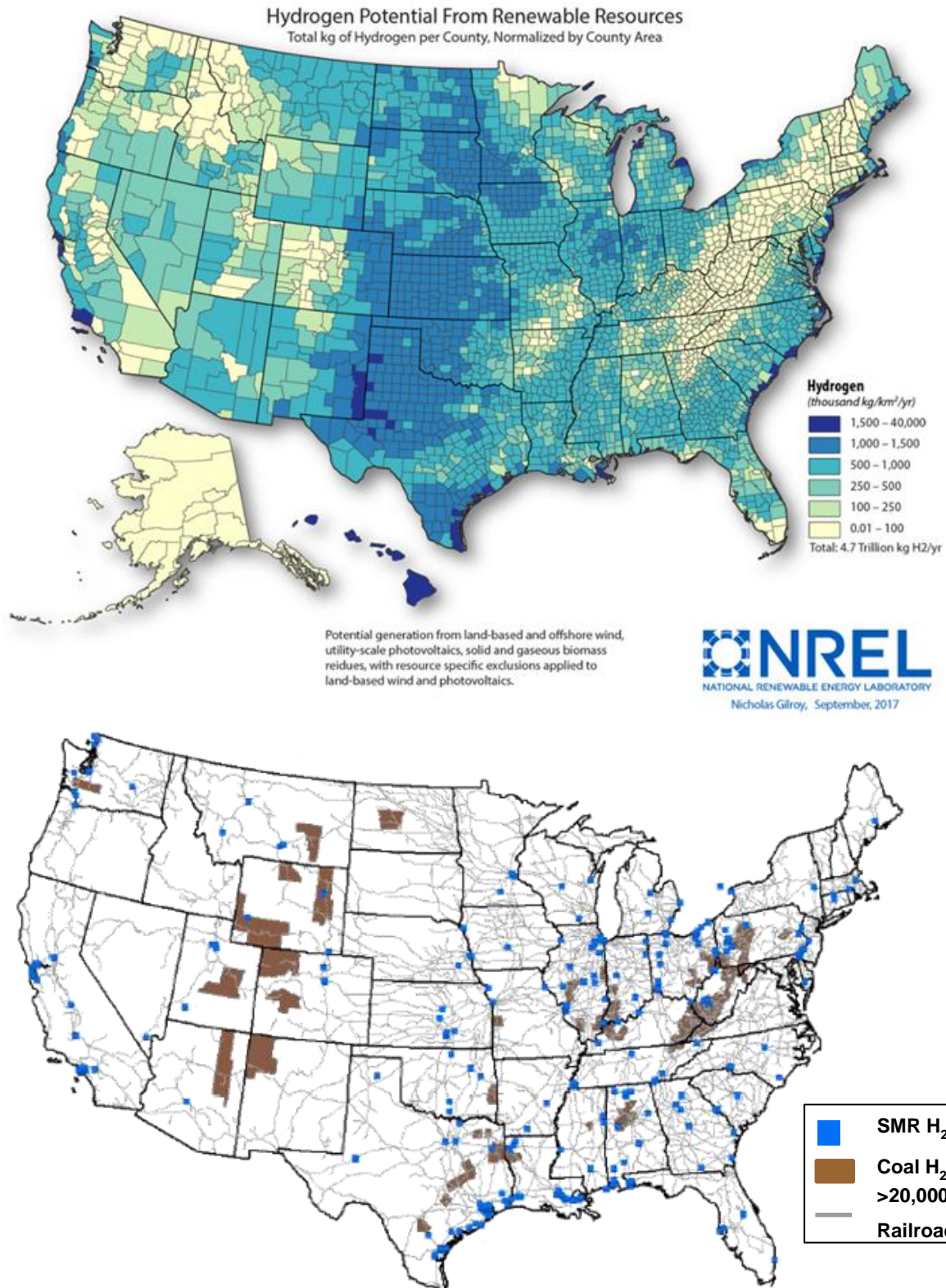
Figure 1 Combined hydrogen production potential from biomass, wind and solar (top) and current hydrogen production from natural gas using steam-methane reforming (SMR) and potential hydrogen production from coal (bottom).
