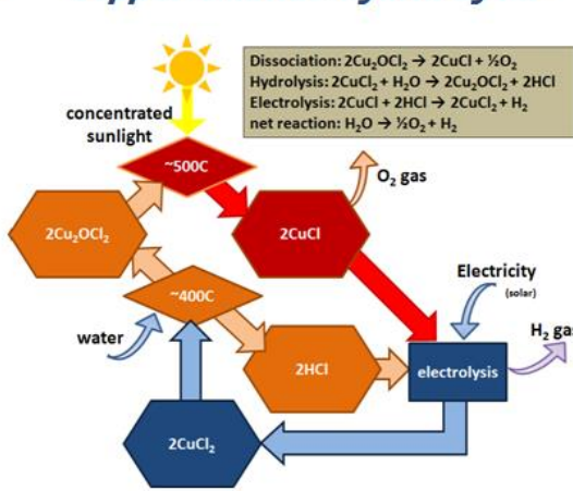
Figure 11 Examples of Solar Thermochemical Cycles for Hydrogen Production.
