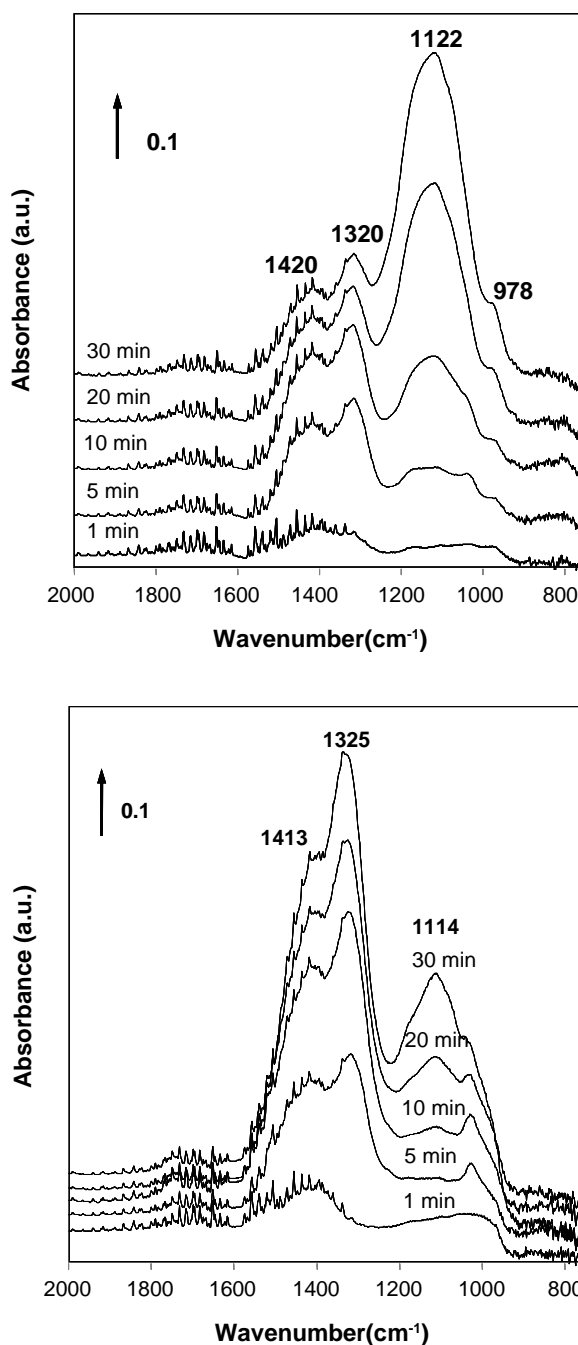
FIGURE 1. DRIFT Spectra Obtained upon Exposure of PBA (top) and PBAC (bottom) to SO 2 /NO/O 2 /H 2 O
