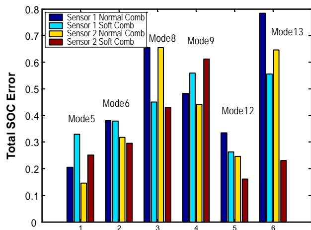
FIGURE 3. Mean SOC Error ( 1\sigma – 0.41 °CA)
