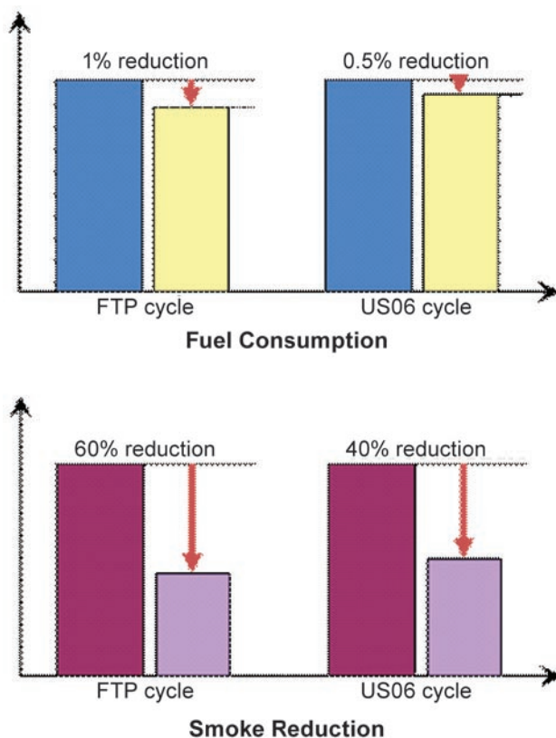
FIGURE 1. Benefits of Using LIRC in a Single-Cylinder Diesel Engine
