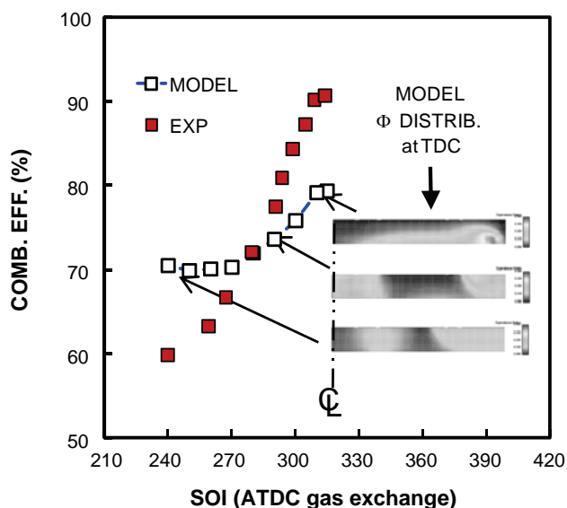
FIGURE 4. Effect of injection timing on HCCI combustion efficiency; SIRD model compared to experimental results of Dec and Sjöberg [4]. Insets are predicted \Phi distributions at TDC showing greater stratification with later injection.
