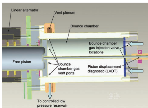
FIGURE 3. Bounce Chamber Gas Dynamometer Operation (Block arrows show gas flow direction.)
