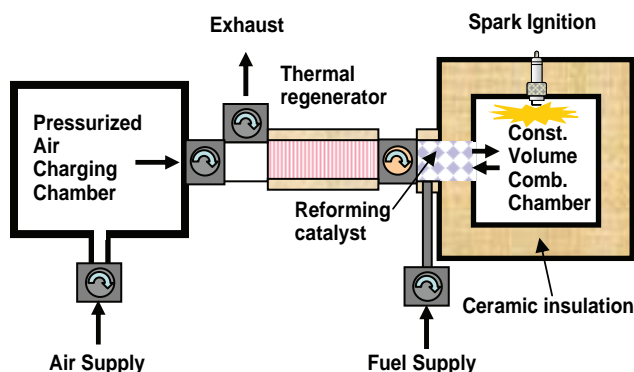
FIGURE 1. Conceptual Design of the RAPTR Experiment
