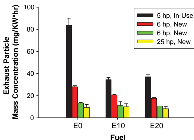
FIGURE 1. Particulate mass emissions for small utility engines operating on intermediate ethanol blends. Note that the older model showed the biggest decrease in emissions.
