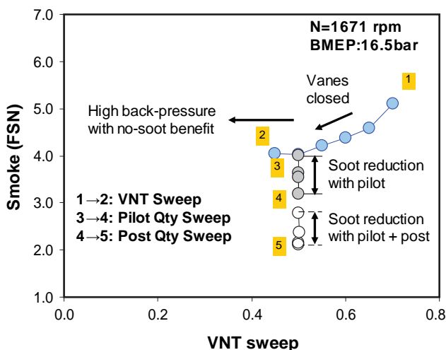
FIGURE 5. Effect of Injection Strategy ( \text{NO}_x = 0.2 \text{ g/bhp-hr} constant; VNT = variable nozzle turbine)
