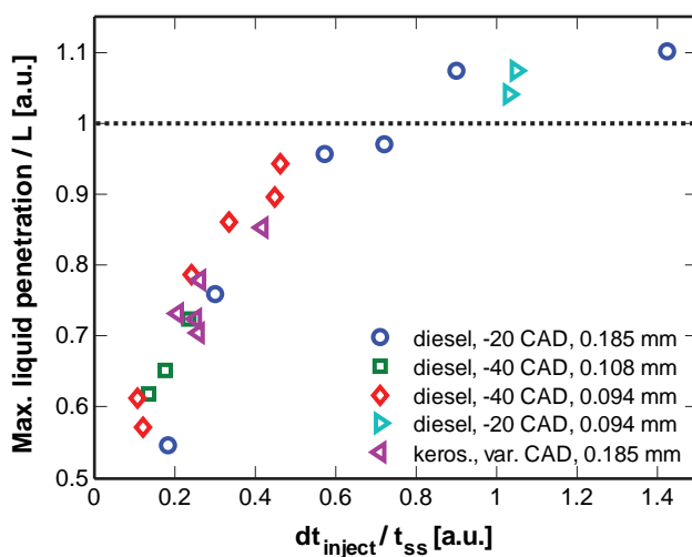
FIGURE 3. Effect of injection duration on liquid penetration. Injection duration is normalized by the time for a spray to reach a steady liquid length at a given condition. The maximum liquid penetration during injection is normalized by the steady liquid length. Various experimental conditions are given in the legend.
