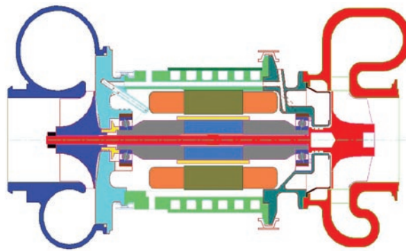
FIGURE 2. Turbogenerator Cross Section
