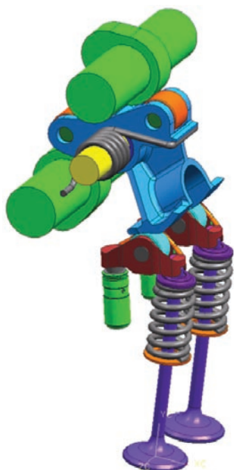
FIGURE 2. Selected Design “A” Continuously Variable Valve Duration
