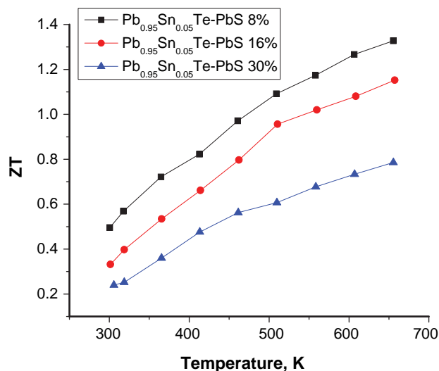
FIGURE 1. Thermodynamic Figure of Merit (ZT) Data Acquired from Individually Prepared Ingots
