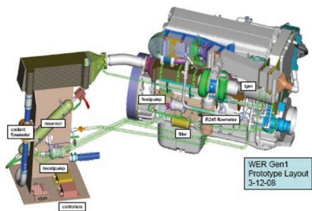
FIGURE 3. Test Cell Hardware Configuration
