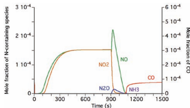
FIGURE 4. Simulated outlet concentrations for a benchmark long storage/regeneration cycle at 400°C.
