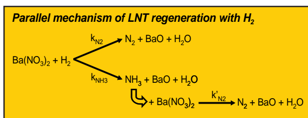
FIGURE 3. Parallel direct- H_2 ( k_{N_2} ) and intermediate- NH_3 ( k_{NH_3} ) regeneration pathways appear feasible. Further work is needed to determine the partitioning between the two regeneration pathways.
