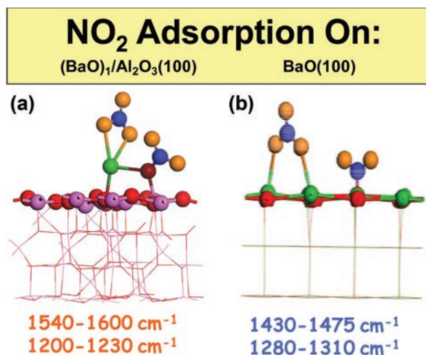
FIGURE 5. Optimized structures of nitrates formed on: a) BaO monomers on the \gamma\text{-Al}_2\text{O}_3(100) surface; and b) a bulk \text{BaO}(100) surface (blue: N; gold: O in \text{NO}_x ; green: Ba; dark red: O in BaO monomer; magenta: \text{Al}^{3+}_{\text{pentar}} ; and red: O atoms on the \text{BaO}(100) and \gamma\text{-Al}_2\text{O}_3(100) surfaces).
