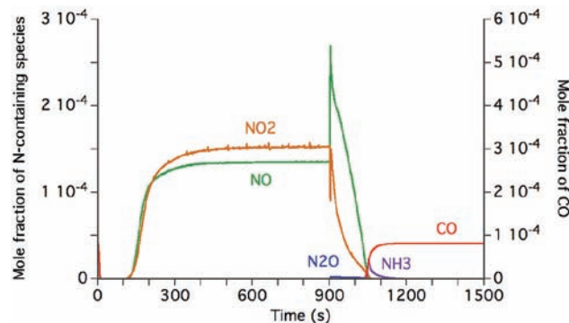
FIGURE 3. Experimental outlet concentrations for a benchmark long storage/regeneration cycle at 400°C [2].
