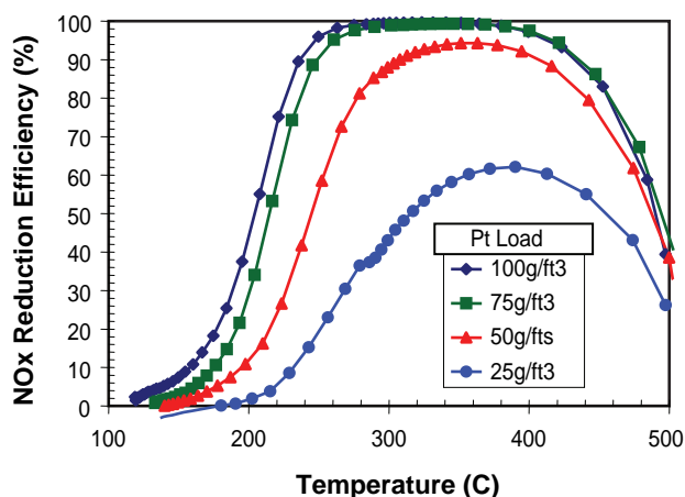
FIGURE 3. NO x Reduction Efficiency as a Function of Temperature for Four Different Pt Loadings
