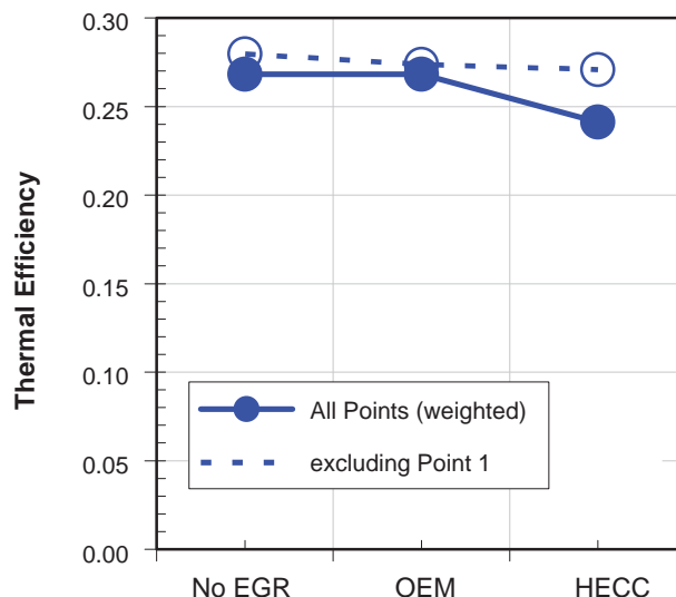
FIGURE 4. Estimated Thermal Efficiency Based on the Same Weighted Steady State Data Shown in Figure 3 for all Combustion Modes
