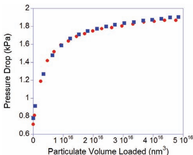
FIGURE 1. Reproducibility of Filtration Experiments with Aerosolized Salt Particles
