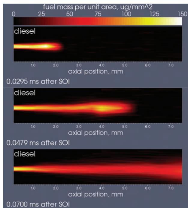
FIGURE 3. Fuel distributions of pure diesel fuel at three different times after start of injection measured under an ambient density of 25 kg/m³. These measurements are the first that have been made without the use of a fuel additive to improve the image contrast.
