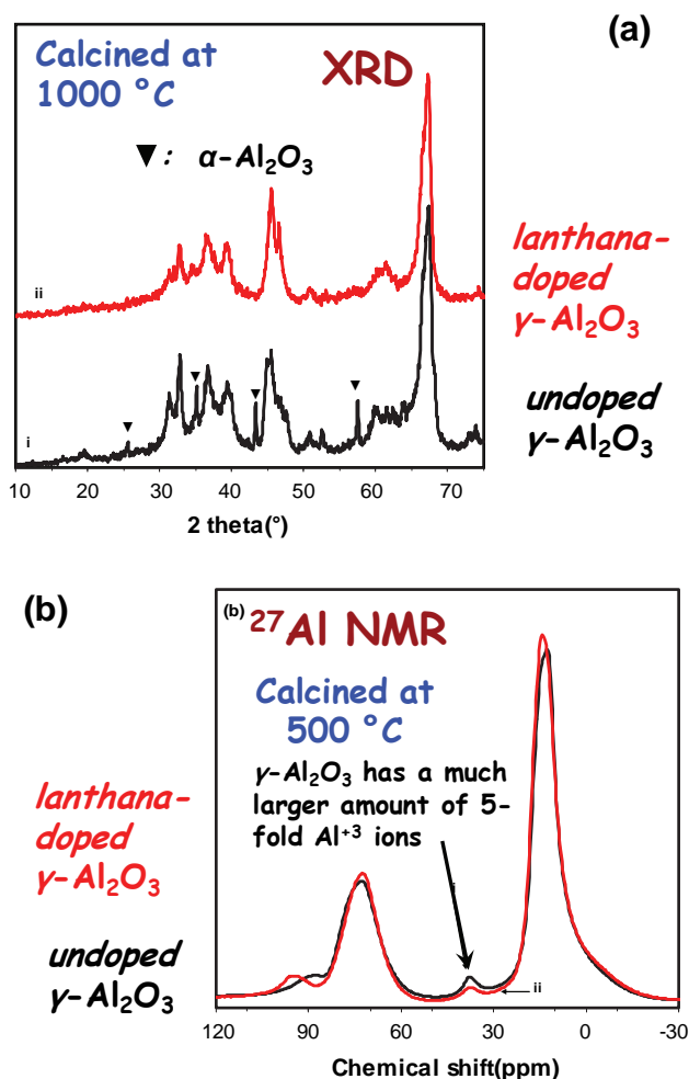
FIGURE 4. XRD patterns (a) after calcined at 1,000°C for 10 h, and solid state ^{27}\text{Al} MAS NMR spectra (b) after calcined at 500°C for 2 h of \gamma\text{-Al}_2\text{O}_3 -150 (black), and \text{La}_2\text{O}_3/\text{Al}_2\text{O}_3 (red) samples.
