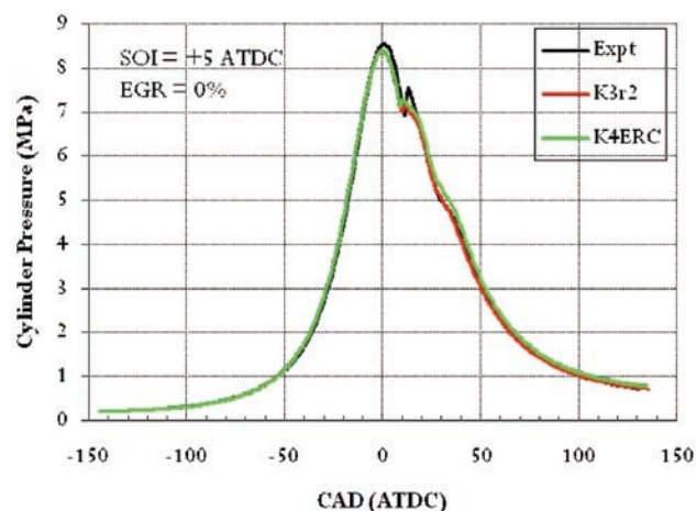
FIGURE 5. KIVA-4, KIVA-3V and Experimental Pressure History Comparison in a 3401 Caterpillar Engine
