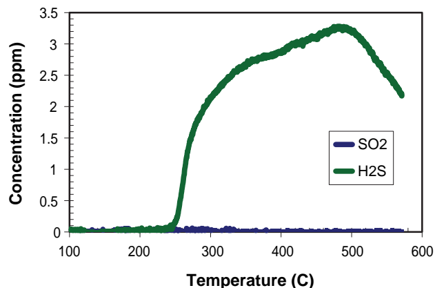
FIGURE 2. TPR Showing Desulfation of the Ce-Based LNT
