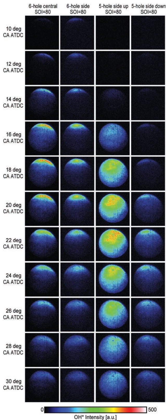
FIGURE 4. Sample OH* intensity plots for different nozzle configurations at high engine load (8 bar IMEP; SOI=80 deg CA BTDC).
