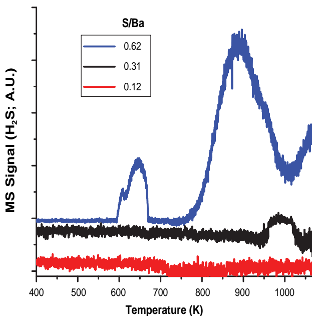
FIGURE 2. \text{H}_2 TRPX spectra for Pt-BaO/ \text{Al}_2\text{O}_3 with different sulfation level, in which is described as \text{S}/\text{Ba} of 0.12, 0.31 and 0.62.
