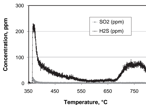
FIGURE 3. Sulfur Release from 20 wt% BaO/ Al_2O_3 + 1 wt% Pt/ Al_2O_3 (1:1 physical mixture) during TPR (1% H_2 , 5% H_2O , 5% CO_2 in Ar)
