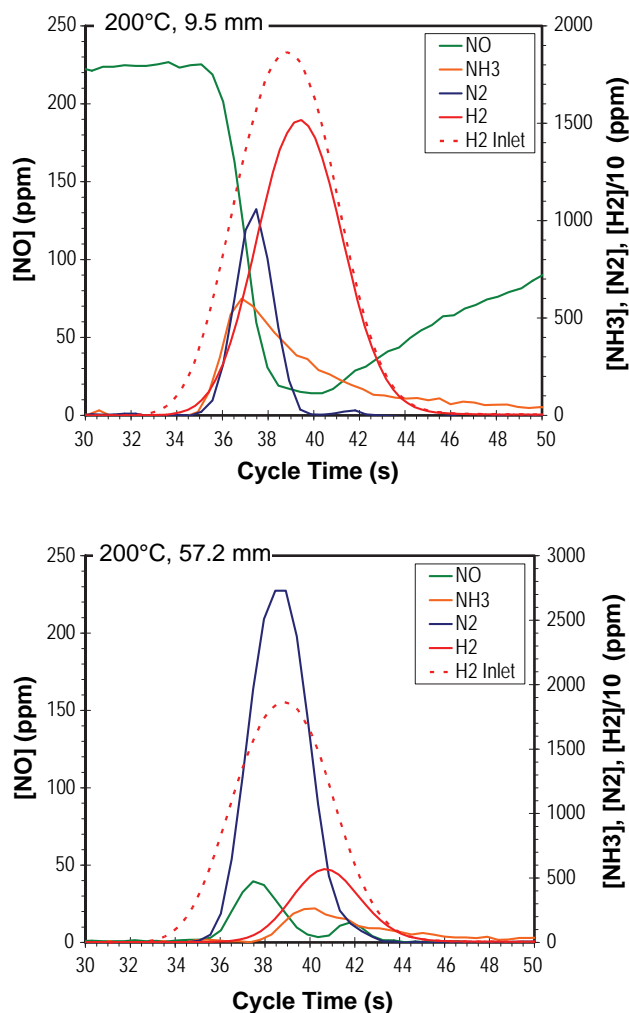
FIGURE 2. Species profiles inside the catalyst channel near the front (9.5 mm) and back (57.2 mm) of the catalyst channel. The species sequence ( N_2 , H_2 \approx NH_3 ) 57 mm along the catalyst channel is typical of the effluent sequence reported in the literature. Measurements at the catalyst front show that in fact NH_3 is generated on the same timescales as is N_2 . However, since N_2 is inert, locally generated N_2 passes unreacted through the catalyst. In contrast NH_3 is continuously being generated and consumed in the NOx-storage region of the catalyst.
