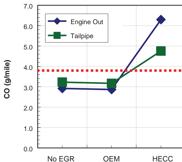
FIGURE 5. Estimated CO Emissions for the FTP Cycle Based On Steady-State Data for all Combustion Modes
