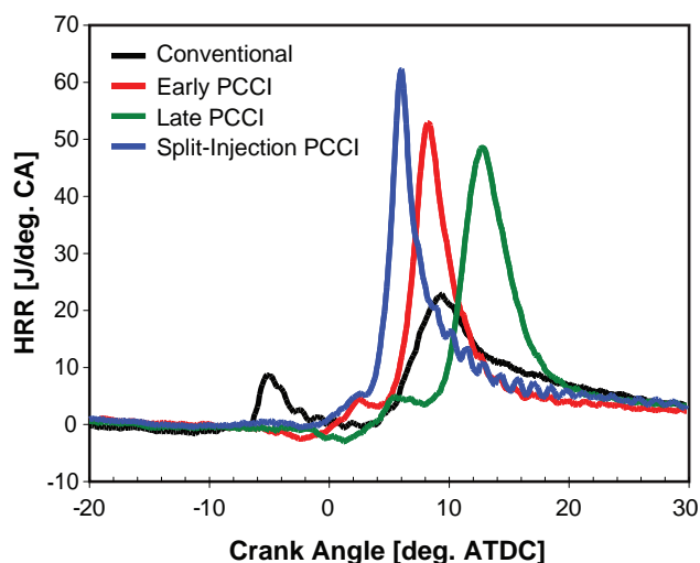
FIGURE 3. Average heat release rate profiles for three HECC strategies and conventional combustion (1,500 rpm/2.6 bar BMEP).
