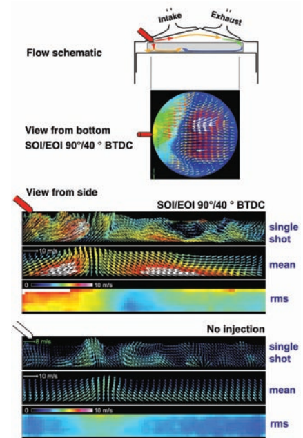
The injection event has a strong influence on the in-cylinder flow, increasing charge velocities of hydrogen engines by more than a factor of two. (Kaiser, SNL)
