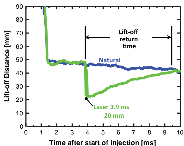
FIGURE 6. Lift-off distance with and without laser ignition for the conditions of Figure 5.
