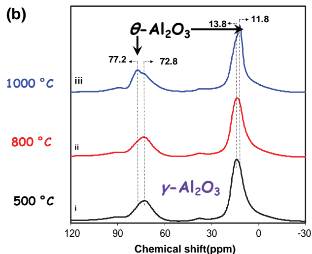
FIGURE 3. XRD patterns (a), and solid state ^{27}\text{Al} MAS NMR spectra (b) of \gamma - \text{Al}_2\text{O}_3 samples calcined at (i) 500°C for 2 h, (ii) 800°C for 2 h, and (iii) 1,000°C for 10 h.
