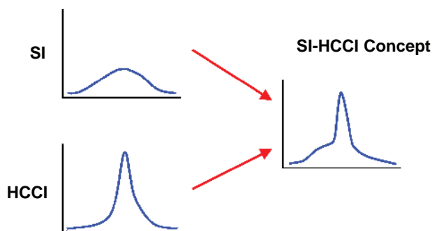
FIGURE 3. Conceptual diagram of the combining of two combustion rate profiles (SI, top left, and HCCI, bottom left) into a composite combustion mode (SI-HCCI, right).
