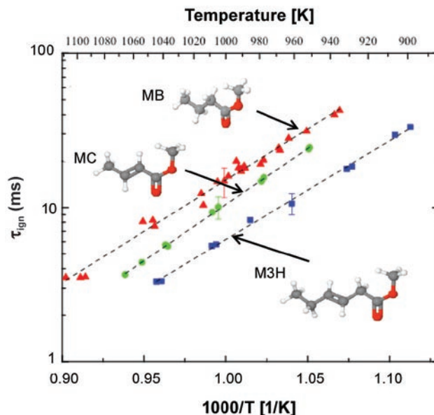
FIGURE 5. Ignition delay times for three biofuel esters measured in the RCF: methyl butanoate (MB) with the longest delay times comparable to isooctane, methyl crotonate (MC), and methyl trans-3-hexanoate (M3H) the most reactive.
