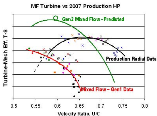
FIGURE 3. Mixed Flow (MF) Turbine Analysis Results
