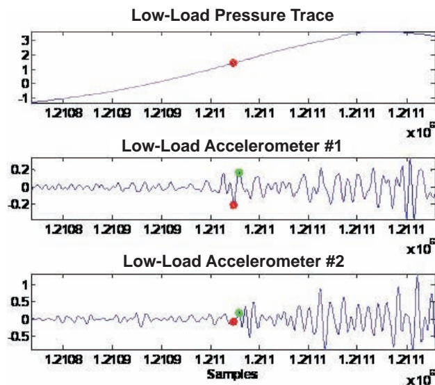
FIGURE 2. Comparison of the identification of the on-line start of combustion using the developed algorithm with the offline research-level approach.
