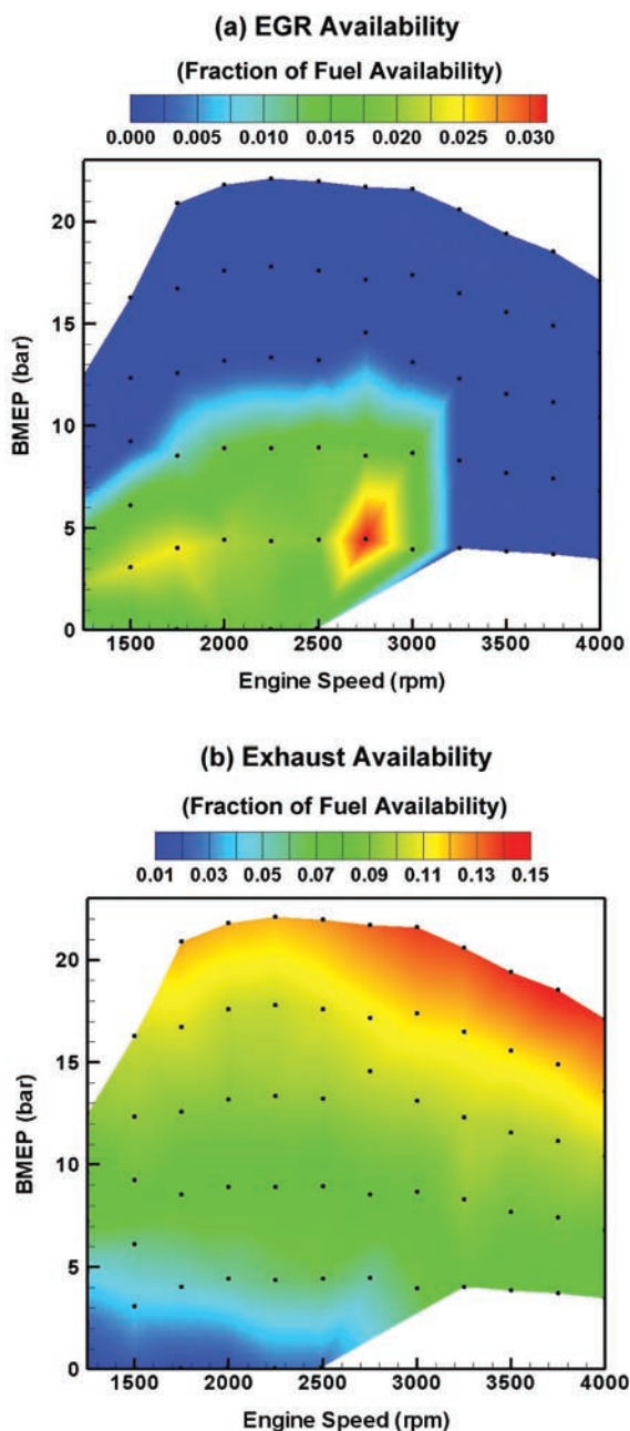
FIGURE 2. Thermodynamic availability of the (a) EGR and (b) exhaust systems on a GM 1.9-L engine shows a significant amount of fuel energy is discarded to the environment and potentially available for recovery.
