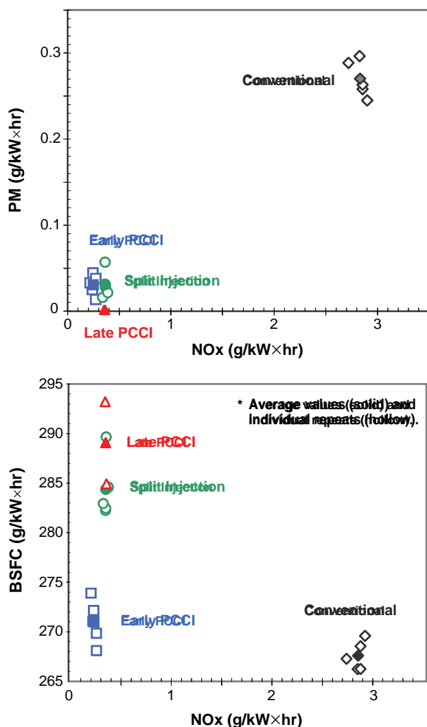
FIGURE 2. Example efficiency and emissions comparison for three HECC strategies and conventional combustion (1,500 rpm/2.6 bar BMEP).
