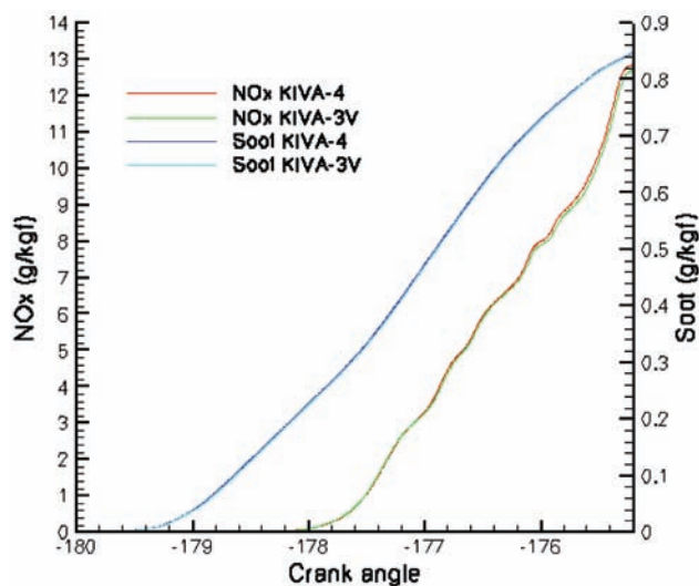
FIGURE 4. Soot and NOx Comparison using KIVA-4 ERC Model and UW-ERC KIVA-3V Model
