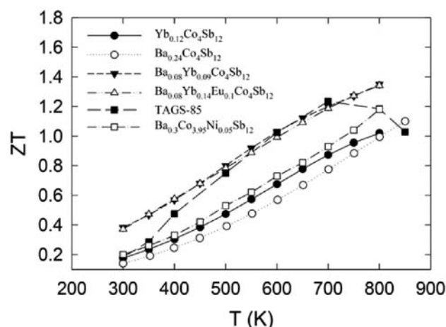
FIGURE 3. Temperature dependence of the ZTs for Ba- and Yb-filled skutterudites [2, 8], double- and triple-filled skutterudites [8], \text{Ba}_x\text{Ni}_{0.05}\text{Co}_{3.95}\text{Sb}_{12} [9], and (\text{AgSbTe})_{2-x}(\text{GeTe})_{0.15} [10]. The accuracy of ZT is estimated to be 20%.
