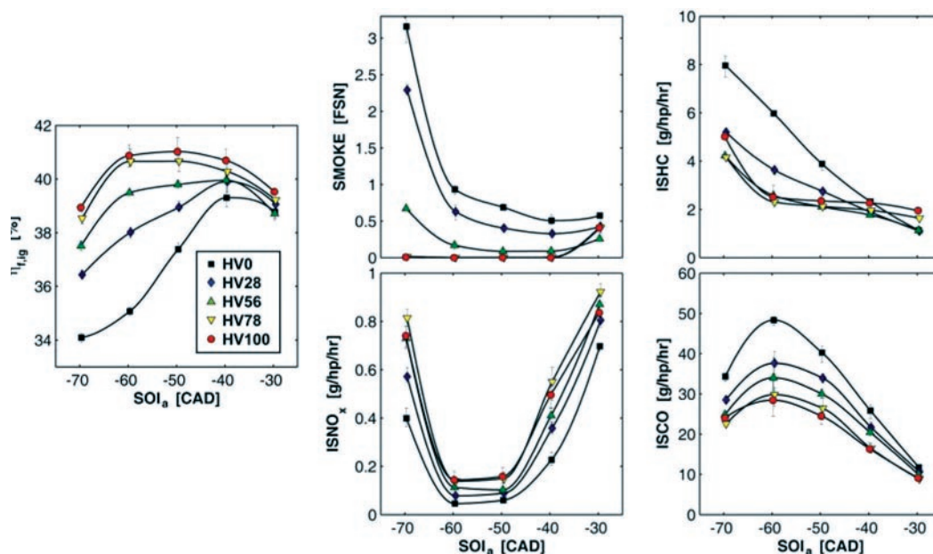
FIGURE 2. Gross indicated fuel-conversion efficiency ( \eta_{fig} ), smoke, and indicated-specific nitrogen oxides (ISNO x ), unburned hydrocarbons (ISHC), and carbon monoxide (ISCO) emissions for HV0, HV28, HV56, HV78, and HV100 over a range of actual start-of-injection (SOI a ) timings. All other operating conditions are the same as those listed in the caption of Figure 1. In general, efficiency increases and smoke, HC, and CO emissions decrease as fuel volatility is increased, while NO x emissions are still compliant with 2010 on-highway truck engine limits for intermediate SOI a timings.
