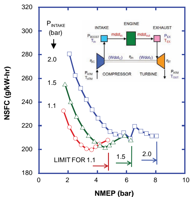
FIGURE 2. Predicted high-load limits and fuel economy using an idealized turbocharger, as computed by the GT-Power ® HCCI model with UM-developed combustion model. (NSFC - net specific fuel consumption)
