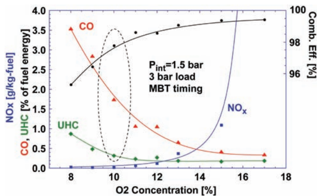
FIGURE 1. Variation in CO, UHC, and combustion efficiency with intake charge O_2 concentration. At the selected operating point, denoted by the dashed ellipse, the global equivalence ratio is about 0.36.
