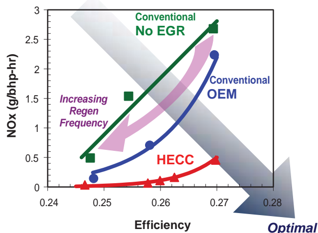
FIGURE 2. NO x Tailpipe Emissions vs. Thermal Efficiency for all Combustion Modes at 2,000 rpm and 2.0 bar BMEP
