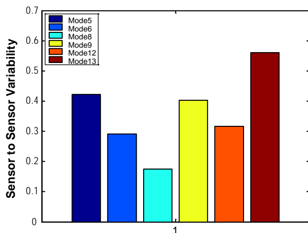
FIGURE 2. Mean Sensor-to-Sensor Variability based on Two Sets of Siemens Knock Sensors ( 3\sigma – 0.36 °CA)
