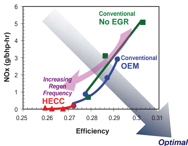
FIGURE 1. NO x Tailpipe Emissions vs. Thermal Efficiency for all Combustion Modes at 1,500 rpm and 2.6 bar brake mean effective pressure (BMEP)
