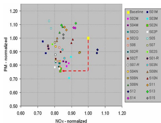
FIGURE 4. Trade-Off of NO x and PM with Advanced Control and Calibration Optimization (Each point marker designates one calibration FTP set point.)
