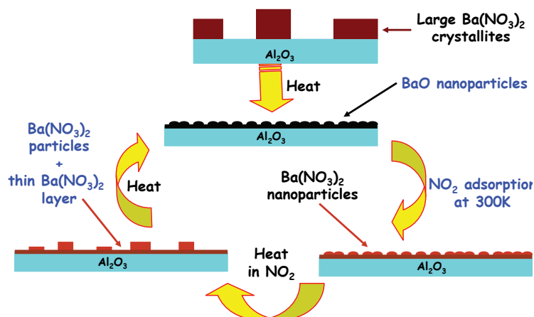
FIGURE 1. Schematics of the cycle of morphology changes taking place during \text{NO}_2 uptake and release on BaO/ \text{Al}_2\text{O}_3 NOx storage/reduction materials.
