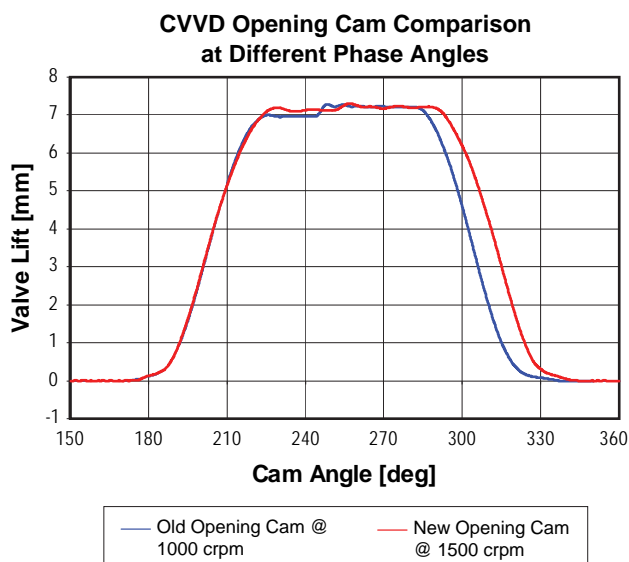
FIGURE 4. Step-Up Comparison of Initial Hardware vs. Modified Opening Cam
