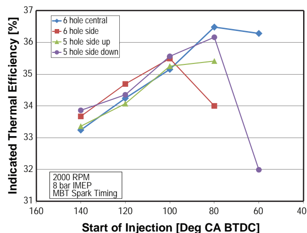
FIGURE 2. Indicated thermal efficiency as a function of start of injection at high engine load (8 bar IMEP).
