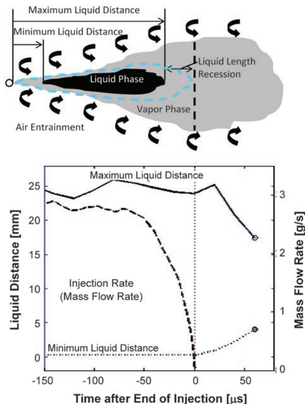
FIGURE 4. Maximum and minimum liquid penetration distances along with a fuel mass flow rate before and after EOI. Schematic of liquid length recession after the end of injection. Ambient conditions: 850 K, 14.8 kg/m 3 0% O 2 . Injector conditions: 0.090 mm nozzle, 150 MPa, #2 diesel.
