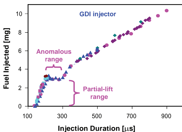
FIGURE 1. Injector fuel delivery for a fuel pressure of 100 bar measured for a range of motored operating conditions.
