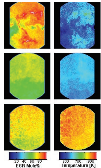
Simultaneous single-shot EGR and temperature images recorded during NVO operation. (Steeper, SNL)
