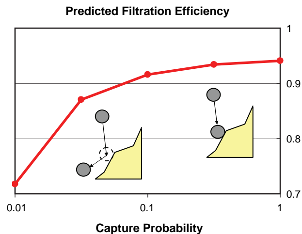
FIGURE 5. Predicted Filtration Efficiency as a Function of Capture Probability
