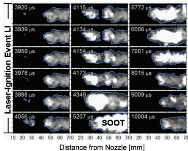
FIGURE 5. Chemiluminescence image sequence with laser ignition at 3.9 ms ASI. Conditions the same as Figure 4, except 21% O 2 .
