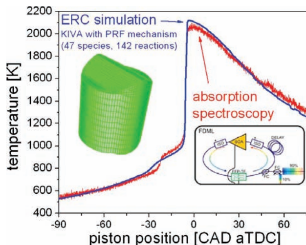
FIGURE 1. Temperature measured by hyperspectral water absorption spectroscopy compared with KIVA PRF fuel model predictions. The temperature measurement has an unprecedented precision of 0.1% (2 K at 2,000 K). (aTDC - after top dead center)
