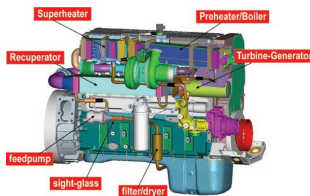
FIGURE 1. Cummins ISX Engine Shown with EGR-Only WHR System Hardware
