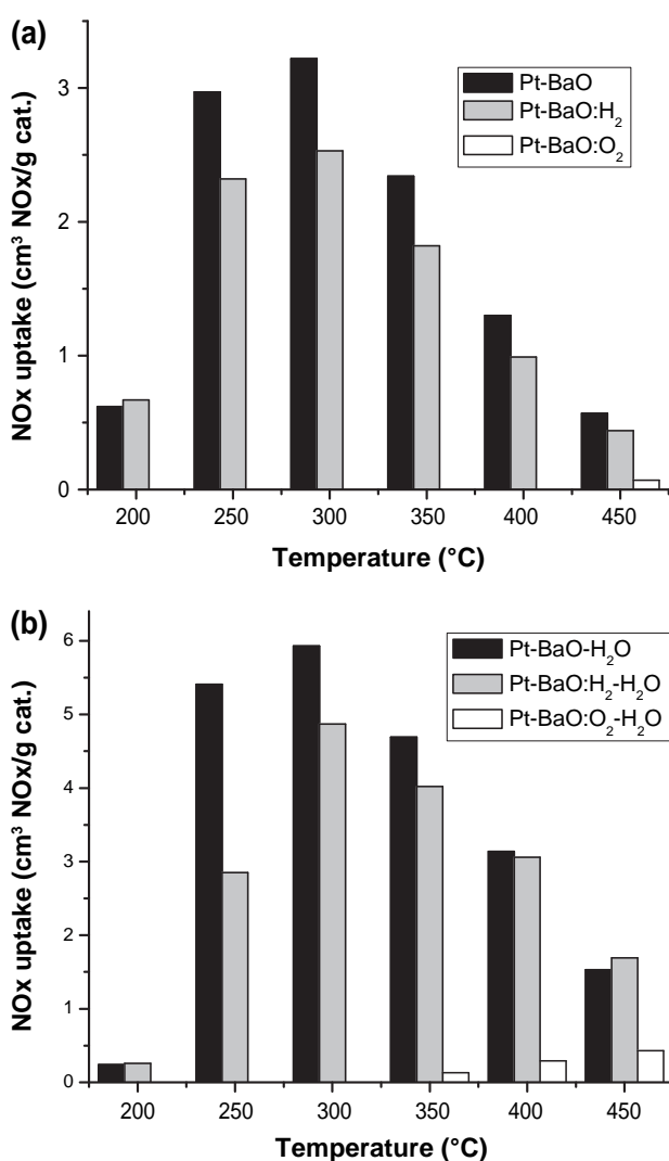
FIGURE 1. Comparison of \text{NO}_x uptake as a function of temperature up to 20% breakthrough of the inlet \text{NO} concentration for over Pt-BaO/ \text{Al}_2\text{O}_3 , Pt-BaO/ \text{Al}_2\text{O}_3 - \text{H}_2 (thermally aged with \text{H}_2 ) and Pt-BaO/ \text{Al}_2\text{O}_3 - \text{O}_2 (thermally aged with \text{O}_2 ) samples (a) and their water-treated samples (b).
