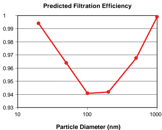
FIGURE 4. Predicted Filtration Efficiency as a Function of Particle Size
