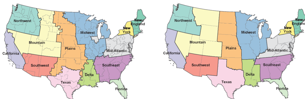
Figure S-7. Geographic regions used to present study results in this analysis. (left) NREL ReEDS modeling zone boundaries shown underlying larger analysis regions. All four NREL studies had this level of granularity. (right) State boundaries underlying larger analysis regions. The Brown & Botterud and Princeton studies had state-level granularity.
