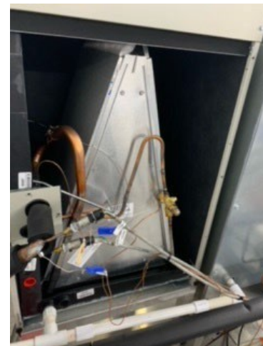
Tested Indoor coil: Option 1: microchannel heat exchange Option 2: tube-fin heat exchanger
