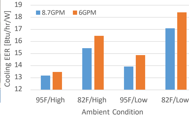
Measured Cooling EER
