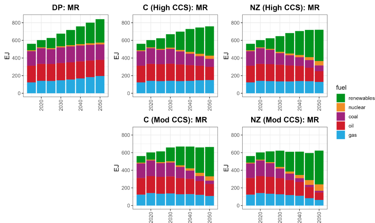
Figure 1. Global primary energy consumption (exajoules, EJ) across scenarios with Model Resolved U.S. LNG export levels.
