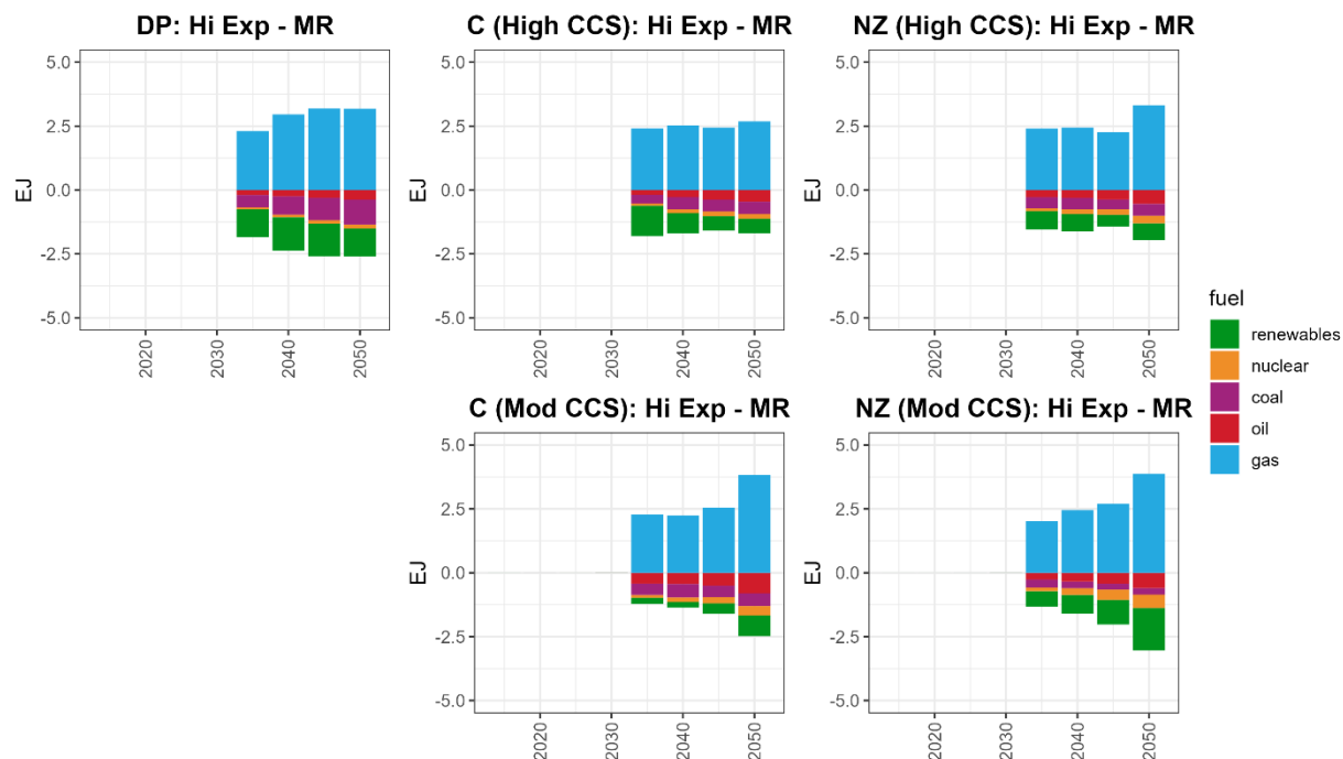
Figure 9. Changes in primary energy consumption in scenarios with High Exports assumptions relative to scenarios with Market Resolved assumptions. DP: MR = Defined Policies: Model Resolved; DP: Hi Exp = Defined Policies: High Exports; C (High CCS): MR = Commitments (High CCS): Model Resolved; C (High CCS): Hi Exp = Commitments (High CCS): High Exports; NZ (High CCS): MR = Net Zero 2050 (High CCS): Model Resolved; NZ (High CCS): Hi Exp = Net Zero 2050 (High CCS): High Exports; C (Mod CCS): MR = Commitments (Moderate CCS): Model Resolved; C (Mod CCS): Hi Exp = Commitments (Moderate CCS): High Exports; NZ (Mod CCS): MR = Net Zero 2050 (Moderate CCS): Model Resolved; NZ (Mod CCS): Hi Exp = Net Zero 2050 (Moderate CCS): High Exports. The High Exports scenarios can also be compared to the Existing/FID scenarios to quantify the changes from a common baseline. These values are summarized in Table 8.
