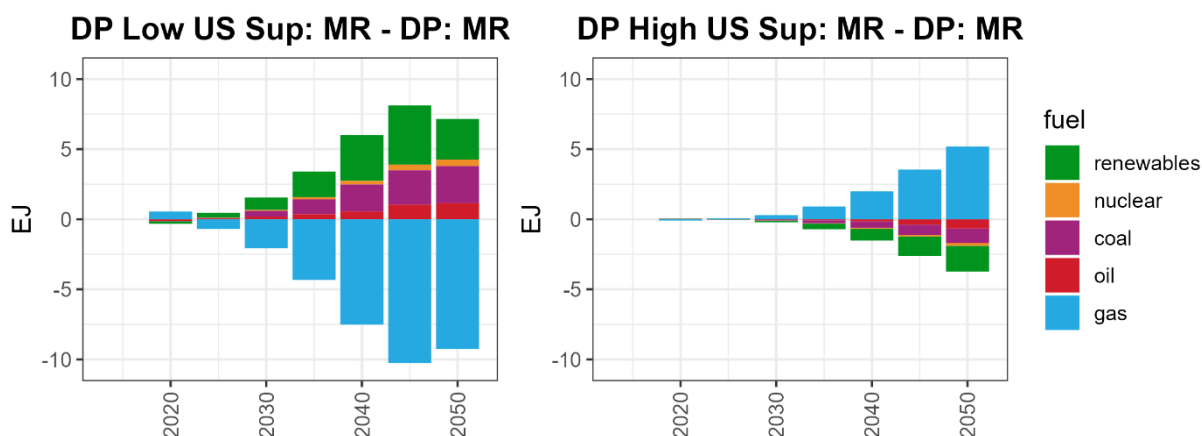
Figure 12. Changes in global primary energy consumption by fuel (EJ) in the DP Low U.S. Supply: Model Resolved and DP High U.S. Supply: Model Resolved scenarios relative to the Defined Policies: Model Resolved scenario. DP: MR = Defined Policies: Model Resolved; DP Hi U.S. Sup: MR = Defined Policies High U.S. Supply: Model Resolved; DP Lo U.S. Sup: Defined Policies Low U.S. Supply: Model Resolved.
