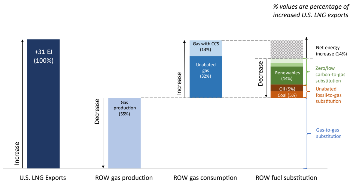
Figure 6. Cumulative changes (2020-2050) in the energy system due to increased U.S. LNG exports in the Commitments (High CCS): Model Resolved scenario relative to the Commitments (High CCS): Existing/FID Exports scenario.
