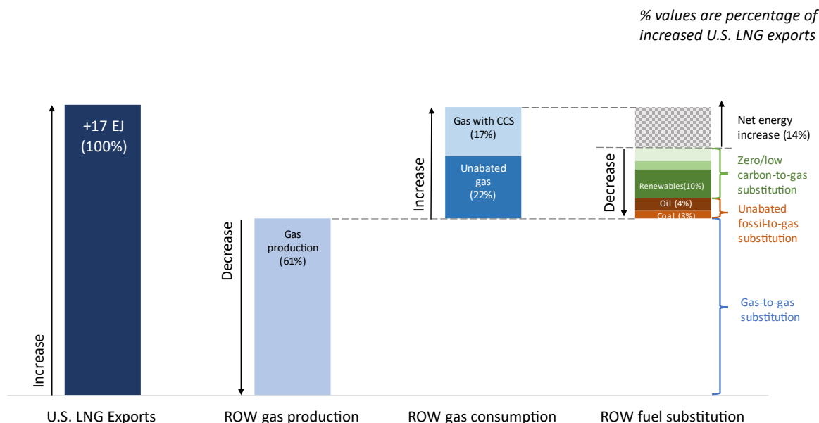
Figure 8. Cumulative changes (2020-2050) in the energy system due to increased U.S. LNG exports in the Net Zero 2050 (High CCS): Model Resolved scenario relative to the Net Zero 2050 (High CCS): Existing/FID Exports scenario.
