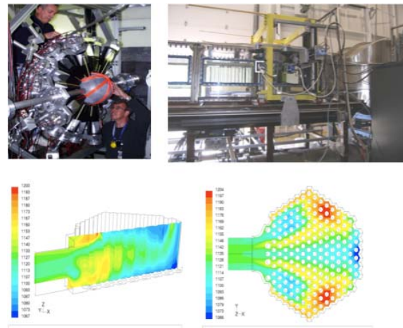
Figure 10. Experiments and Computer Simulations Used in HTGR Design and Safety
