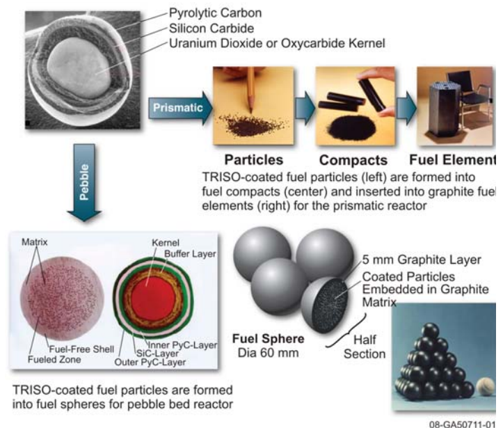
Figure 6. TRISO Coated Particle Fuel
