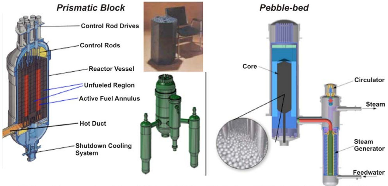
Figure 11. Schematics of the Pebble Bed and Prismatic Designs
