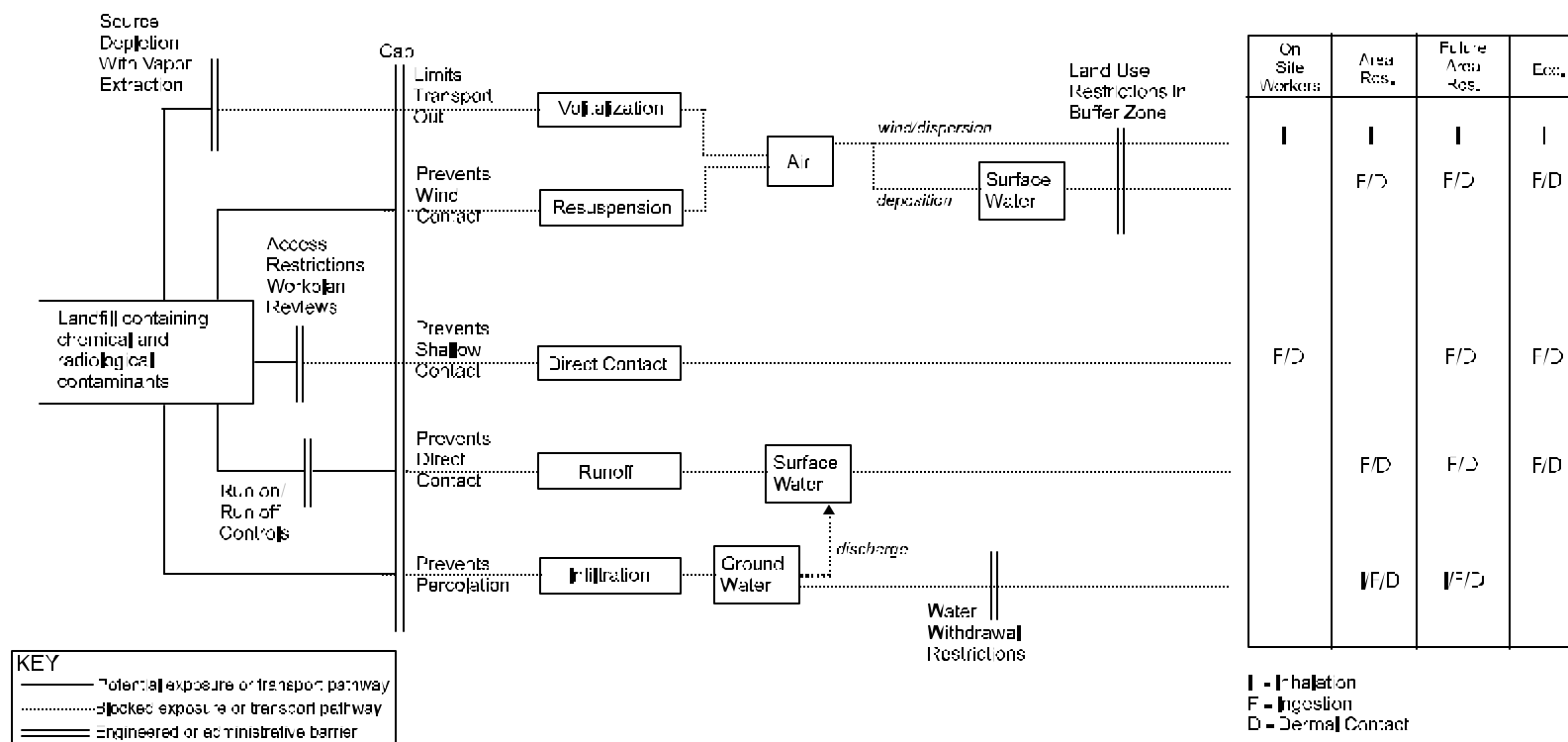
Exhibit G-1. Example of Post-Remediation Conceptual Site Model
