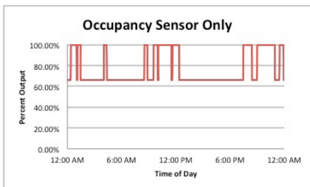
Figure 12. Monitoring for the same structure with an adjacent luminaire only controlled by an occupancy sensor. The sensor reduces the luminaire output by one-third after 20 minutes of no activity detection.
