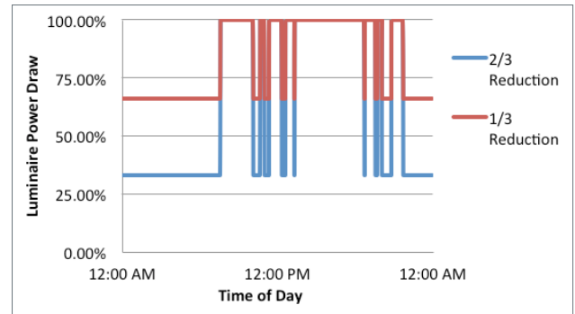
Figure 15. Sample data from an aboveground parking structure supporting an educational campus during the weekday. The figure depicts the usage when the low setting (when no activity is detected) is two-thirds and one-third full power. When the low setting is two-thirds reduction from full power, more energy is saved.
