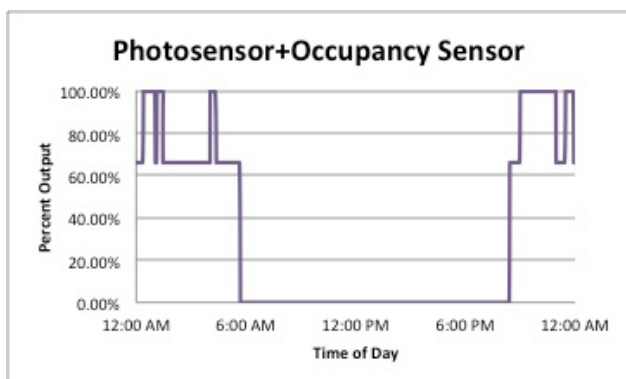
Figure 13. Monitoring for the same structure using both photo and occupancy sensor controls. When daylight is available, the luminaire is off. When it is dark outside, the luminaire is controlled by the occupancy sensor.
