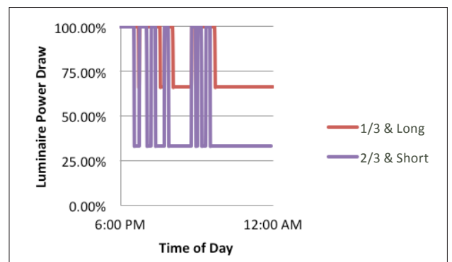
Figure 17. Sample data from an aboveground parking structure supporting an educational campus from 6:00 pm to midnight on a weekday. This graph compares little power reduction and a long time delay to a significant power reduction and a short time delay. Combining the short time delay with the greatest reduction in output permissible can optimize energy savings.
