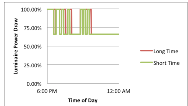
Figure 16. Sample data from an aboveground parking structure supporting an educational campus from 6:00 pm to midnight on a weekday. In the “long time” setting, the luminaire waits for 20 minutes after last activity is detected to go to the low setting. In the “short time” setting, the luminaire waits only for 10 minutes after last activity to go to the low setting. The shorter the time delay, the greater the energy savings.
